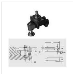
U-Type Special Mould Clamp
