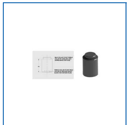
HEIGHT BLOCK FOR LEVELLING JACK
