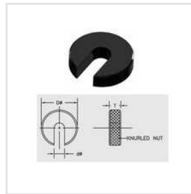
C-Washer
