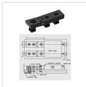
Low High Pinch Clamp
