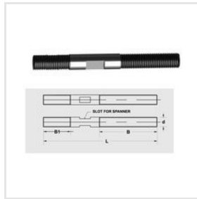
Stud With Slot (Mould Stud)
