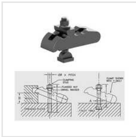
Mould Clamps
