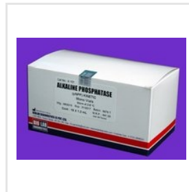
Alkaline Phosphatase
