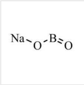
Sodium Metaborate
