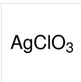
Silver Chlorate
