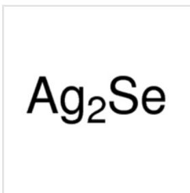
Silver Selenide
