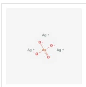
Silver Arsenate
